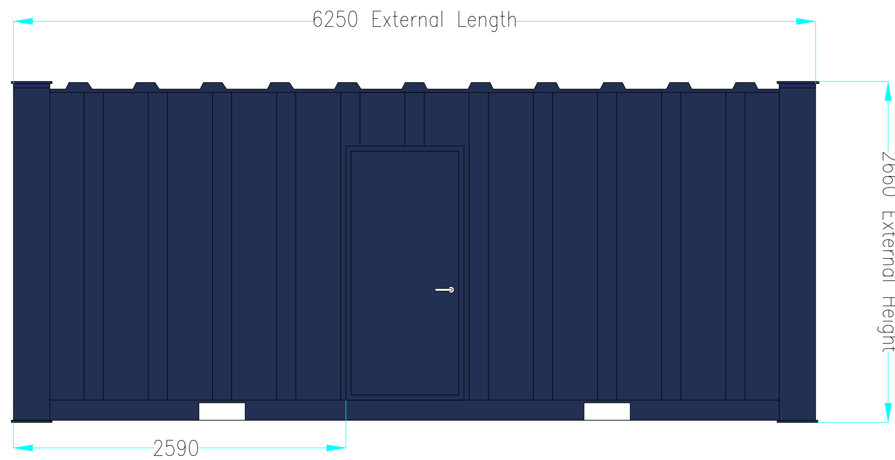
SIDE ELEVATION "A"
