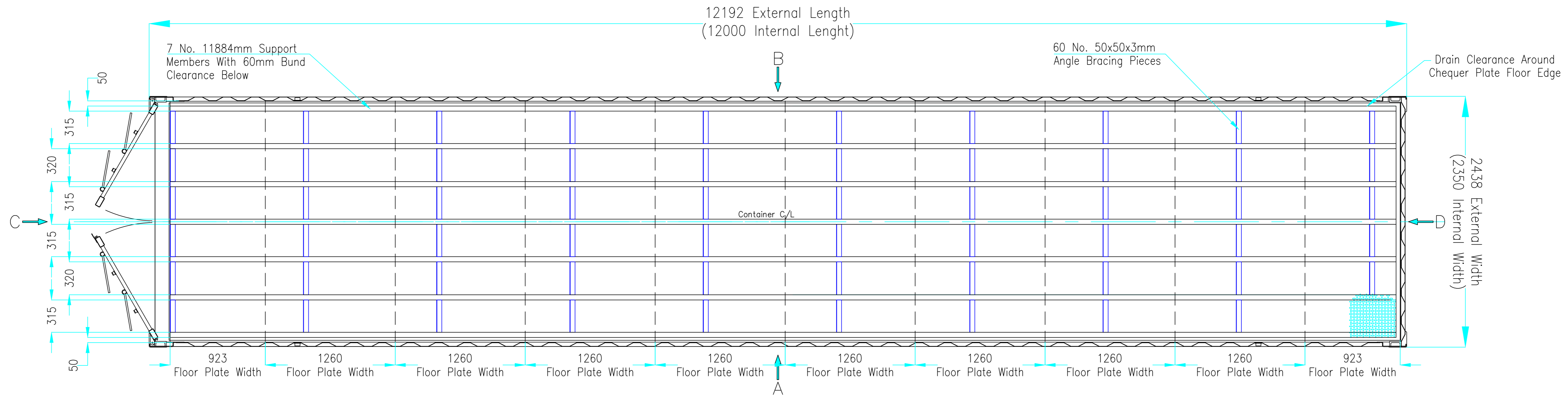
SECTIONAL PLAN
