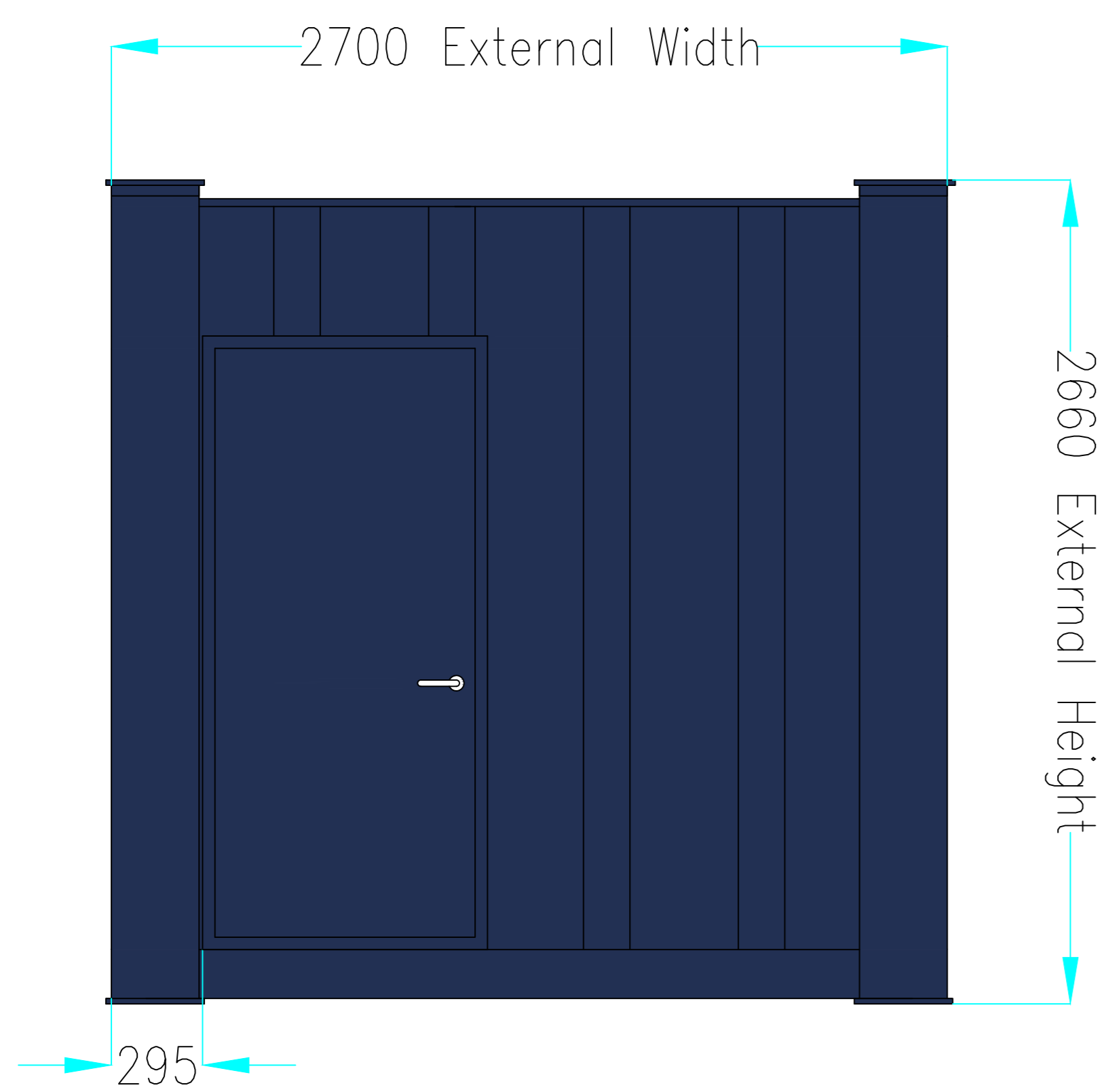
SIDE ELEVATION "C"
