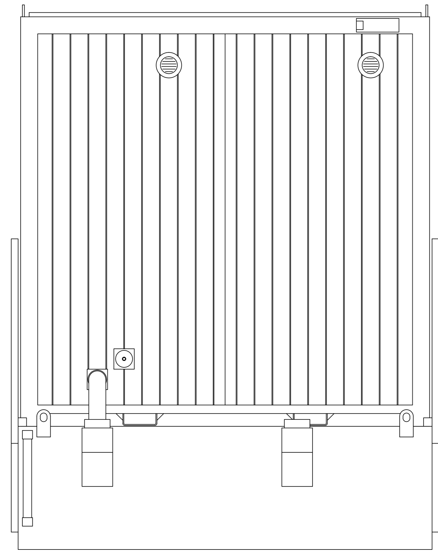
SIDE ELEVATION "C"
