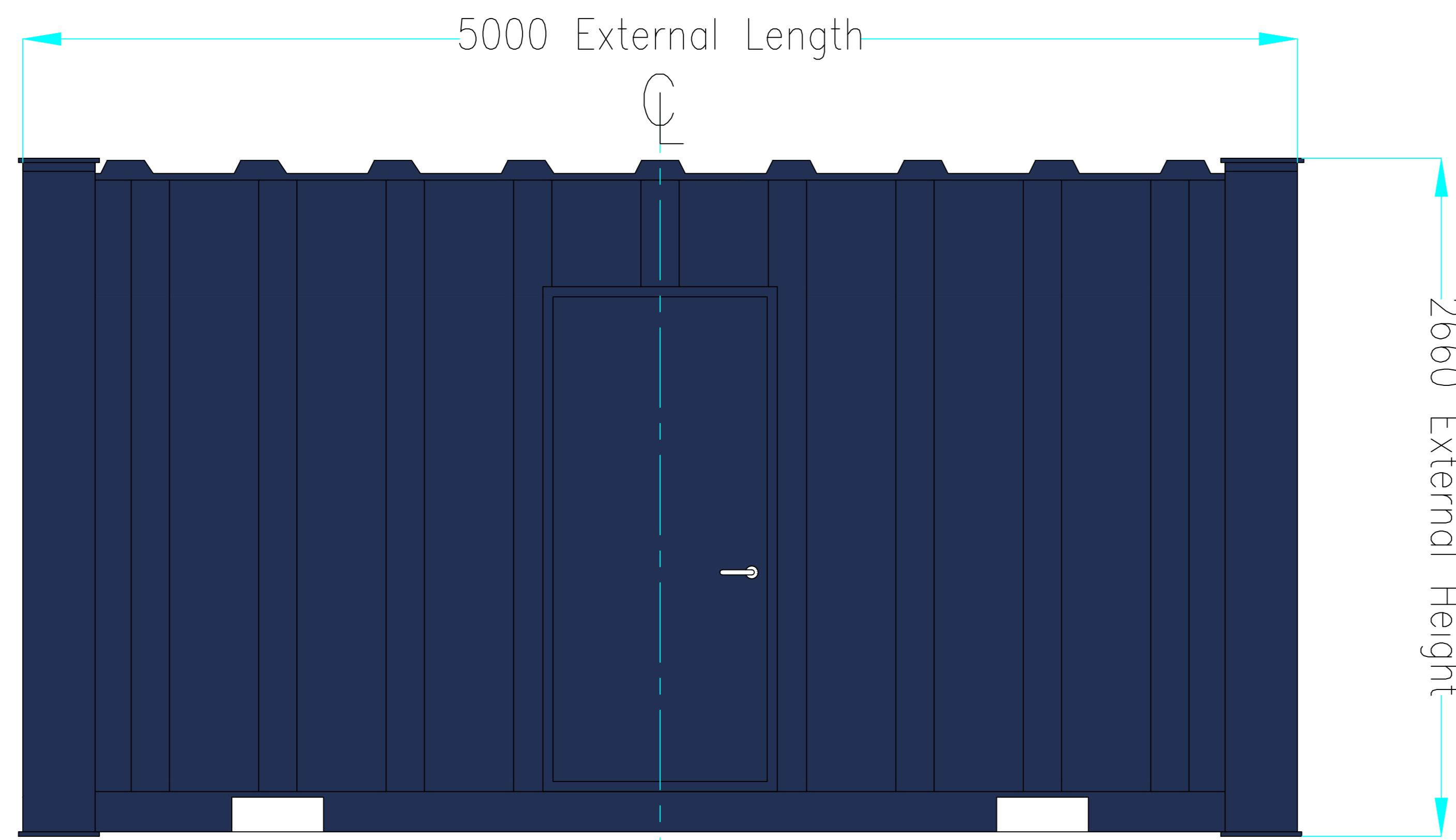
SIDE ELEVATION "A"
