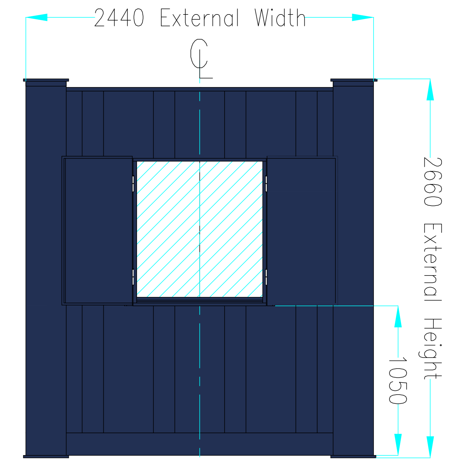
SIDE ELEVATION "D"
