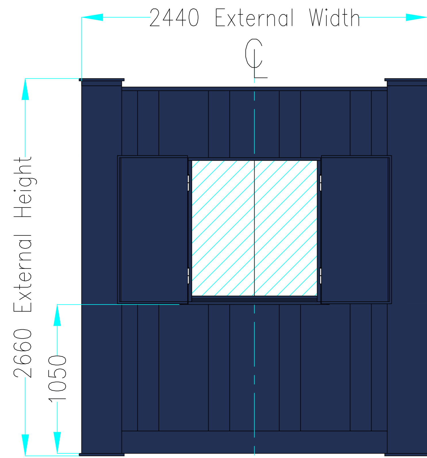
SIDE ELEVATION "C"
