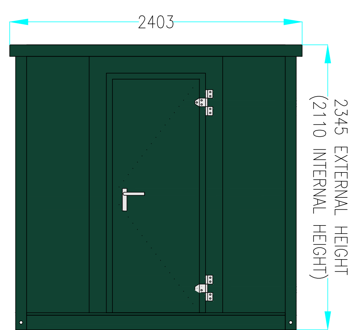
SIDE ELEVATION "C"
